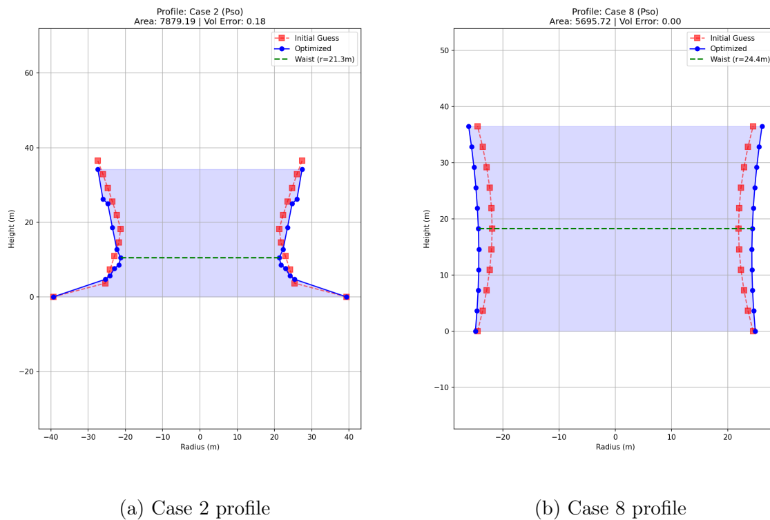
Figure 10: Optimised tower profiles (Cases 2 and 8)
